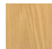
Natural
